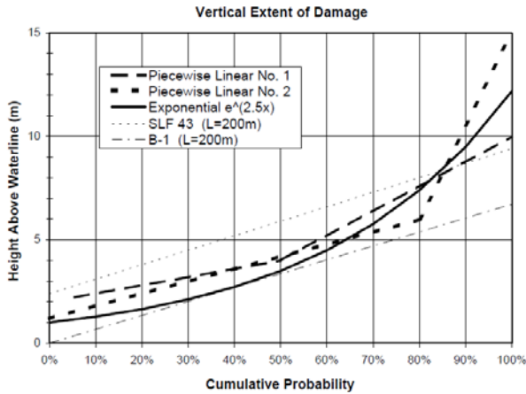
Fig. 1 - Proposals for alternative “v” formula [5]
