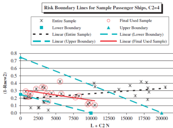
Fig 5 - Risk assessment of passenger ship [8]
