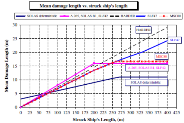
Fig. 2 - Mean Damage Length [8]
