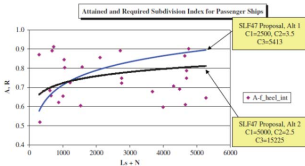
Fig 4 - R-index proposals for passenger ships [8]
