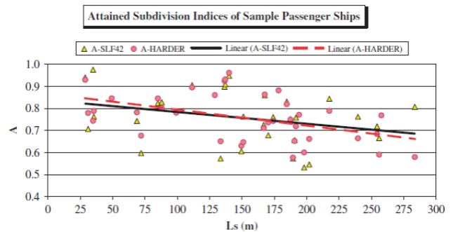
Fig 3 - Attained indices of passenger ships vs. length [8]
