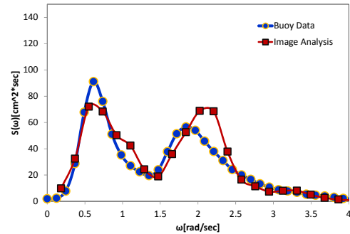
Figure 3.6: The power spectrum of measured vertical displacement of the buoy and analyzed data from the image of buoy motion.
