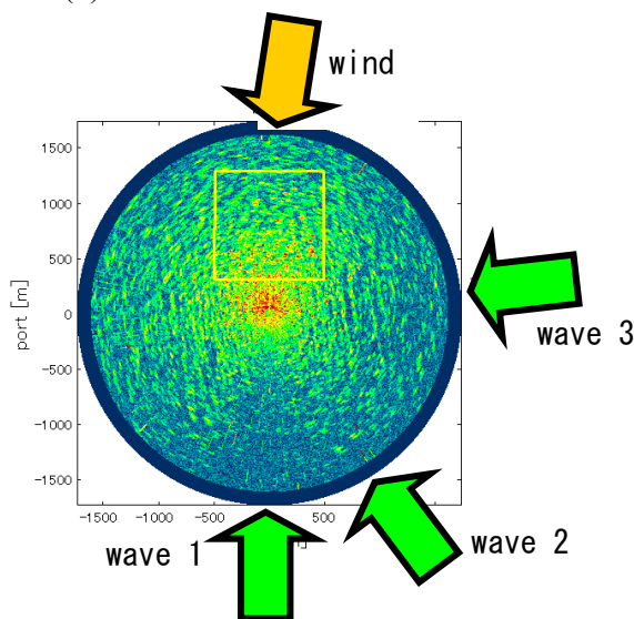
Figure 3.9: Example of PPI image of a radar (Jun.14 2012 12:46). Bow up expression.
