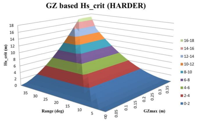
Figure 4: GZ-based H_{s,crit}
